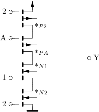
Schematic (one stage, 2T_p/2T_n stacked, 12T total)
