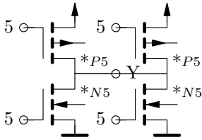
Schematic (one stage, 1T_p/1T_n stacked, 24T total)
