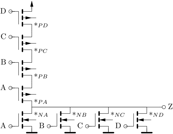
Schematic (two stage, 4T_p/1T_n stacked, 10T total)
