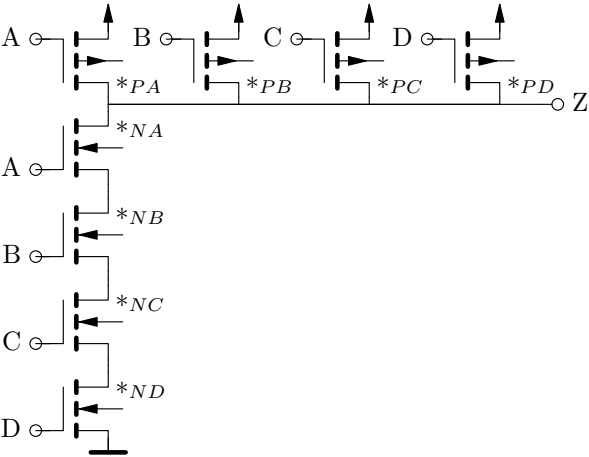
Schematic (two stage, 1T_p/4T_n stacked, 10T total)
